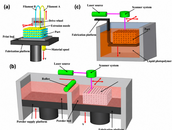
Figure 2. SLA uses a laser to polymerize liquid photopolymer resin SLA: Stereolithography
